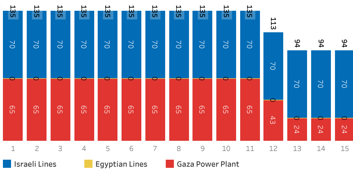
Electricity supply (megawatts per day)
